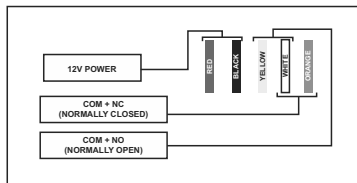
WIRING DIAGRAM
