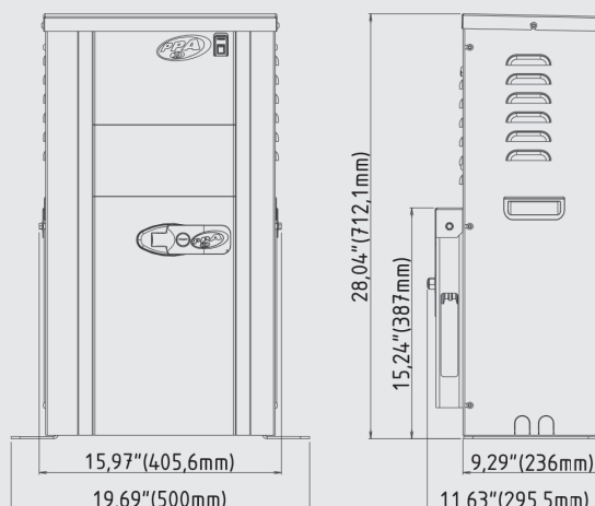
Equipment dimensions
